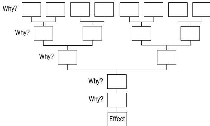
Figure 9.7 Tree Diagram
