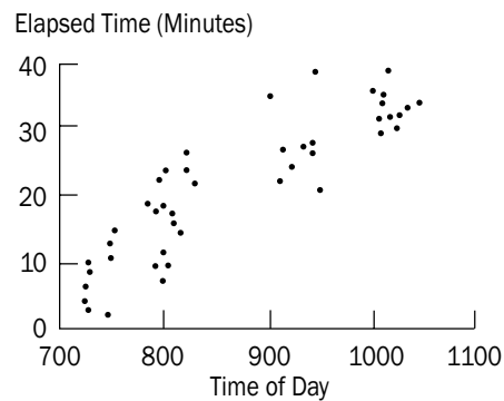
Figure 9.13 Scatter Diagram
