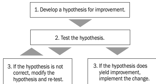
Figure 2.9 Hypothesis Testing
