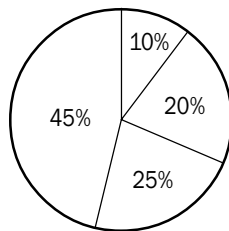
Figure 9.9 Pie Chart
