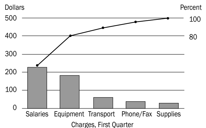
Figure 9.15 Pareto Chart
