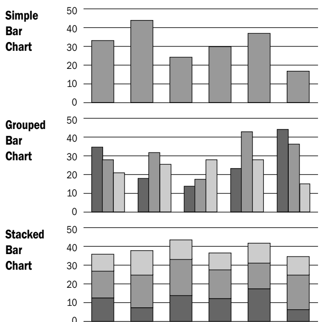
Figure 9.8 Bar Charts
